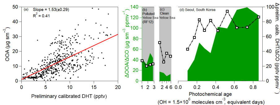
Figure 8. (a) Scatter plot of OOA versus DHT over Seoul, South Korea, during KORUS-AQ, after 12:00 LT (03:00 UTC). (b) Same as Fig. 7g, but for DHT over the Yellow Sea (RF12). (c) Same as Fig. 7h, but for DHT over the Yellow Sea. (d) Same as Fig. 7i, but for DHT over Seoul. As an important note, concentrations of DHT are based on a preliminary calibration; however, any further calibrations are not expected to impact the relative trend and general correlation.
